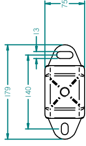
AVM MOUNT DETAILS
